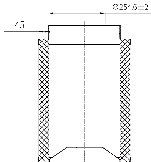
Internal Carbon Filter Cross-Section
