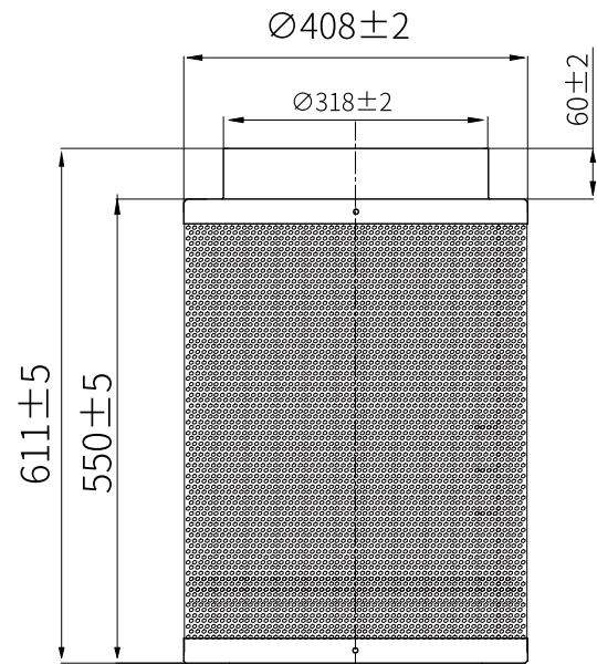
Internal Carbon Filter Dimensions
