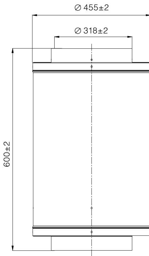
Complete Unit Dimensions
