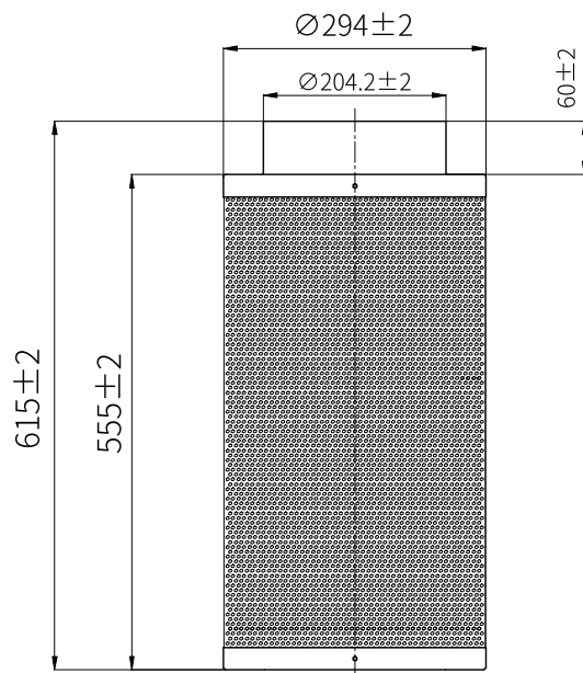
Internal Carbon Filter Dimensions
