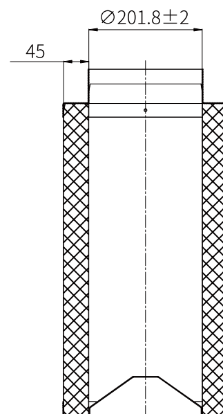
Internal Carbon Filter Cross-Section
