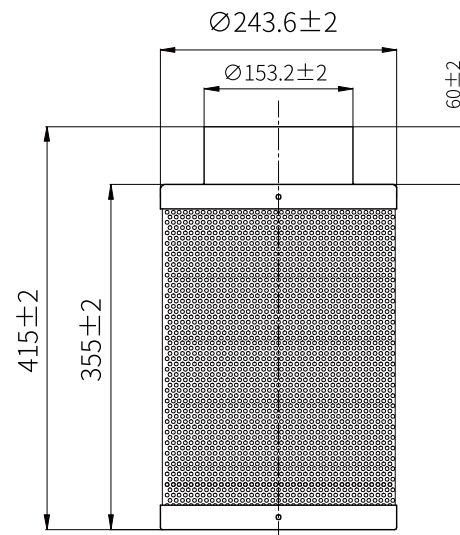
Internal Carbon Filter Dimensions
