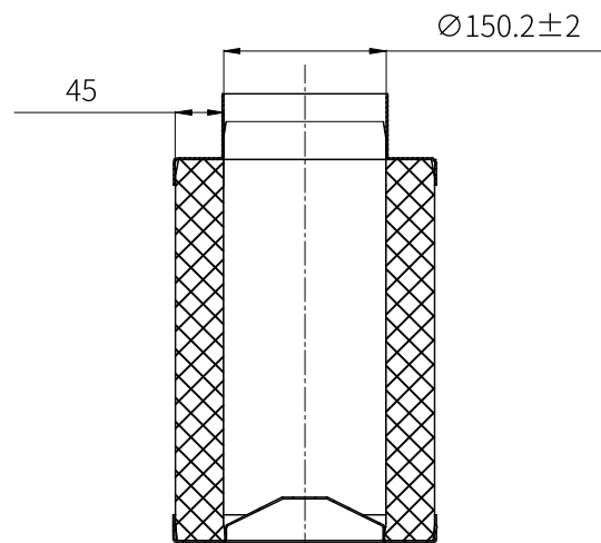
Internal Carbon Filter Cross-Section
