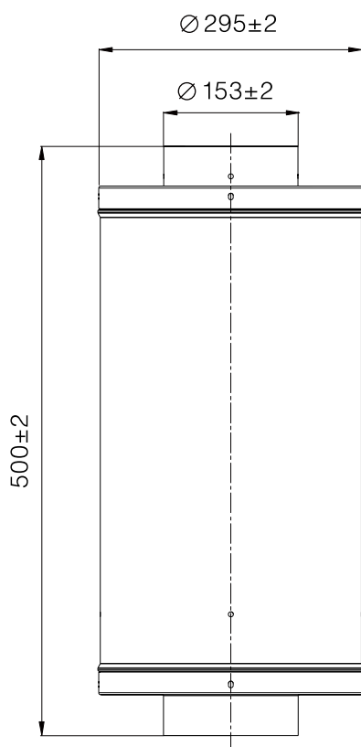
Complete Unit Dimensions
